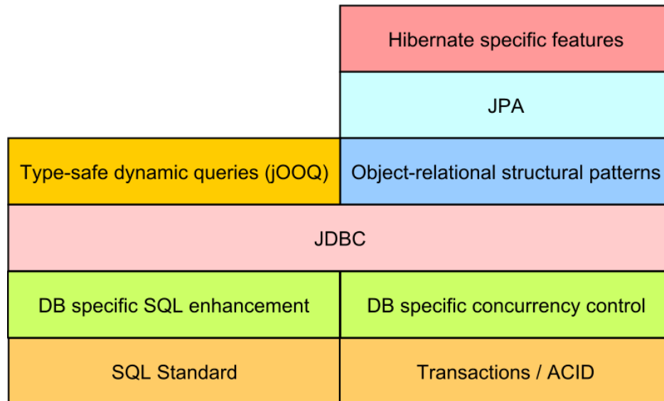
Figure I.1: Data access skill stack
