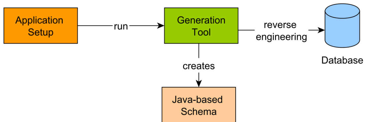
Figure 17.1: Java-based schema generation
