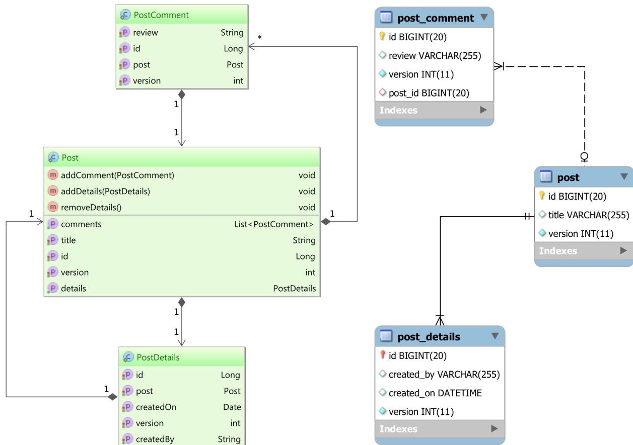
Figure 7.1: Object/Relational Mapping
