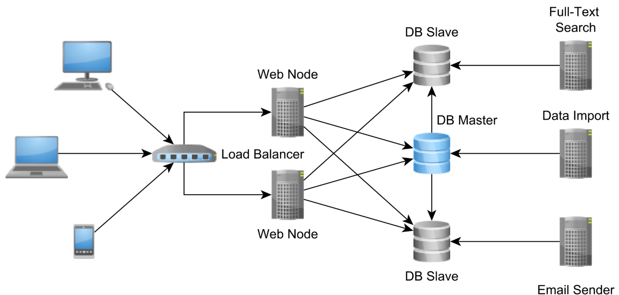
Figure 7.2: Database-centric integration
