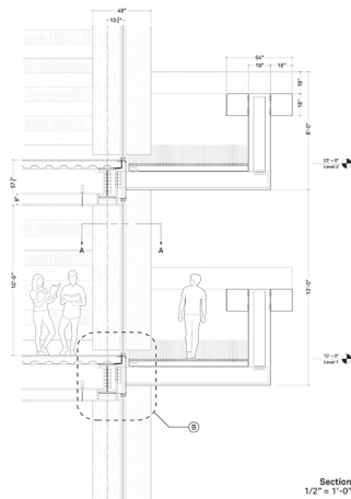
Section 1/2" = 1'-0"
