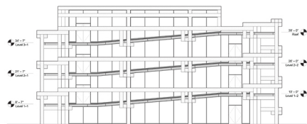
South Elevation 1/8" = 1'-0"
