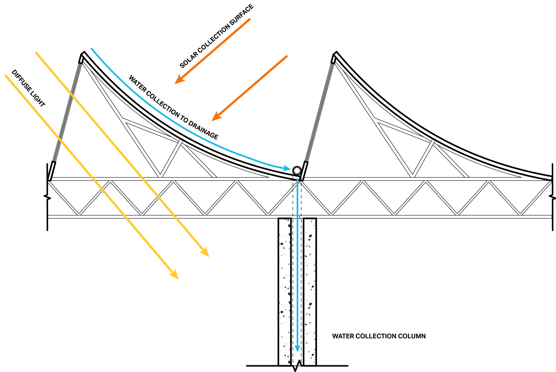
SOLAR SAWTOOTH ROOF DETAIL
