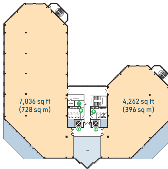
FIRST FLOOR 12,098 sq ft (1,124 sq m)
