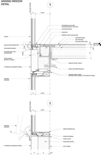
3. AWNING WINDOW DETAIL
