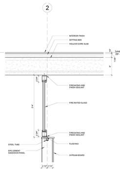
2. INTERIOR HALLWAY PARTITION WALL DETAIL
