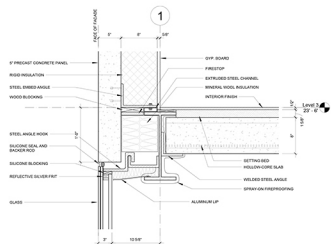
1. HALLWAY FULL-HEIGHT GLAZING DETAIL
